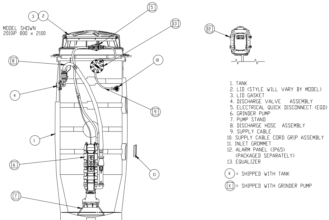
Fig. 1 - Station Components
