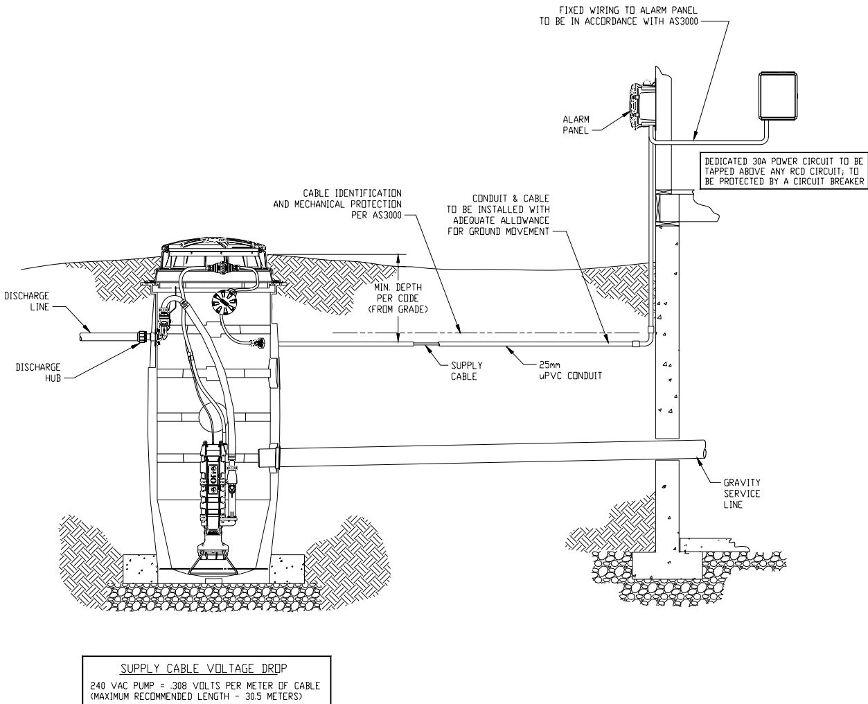
Fig. 6 - Typical Station Installation
