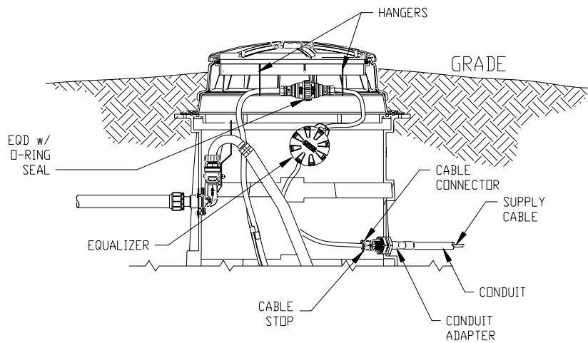
Fig. 7 - Electrical Cables
