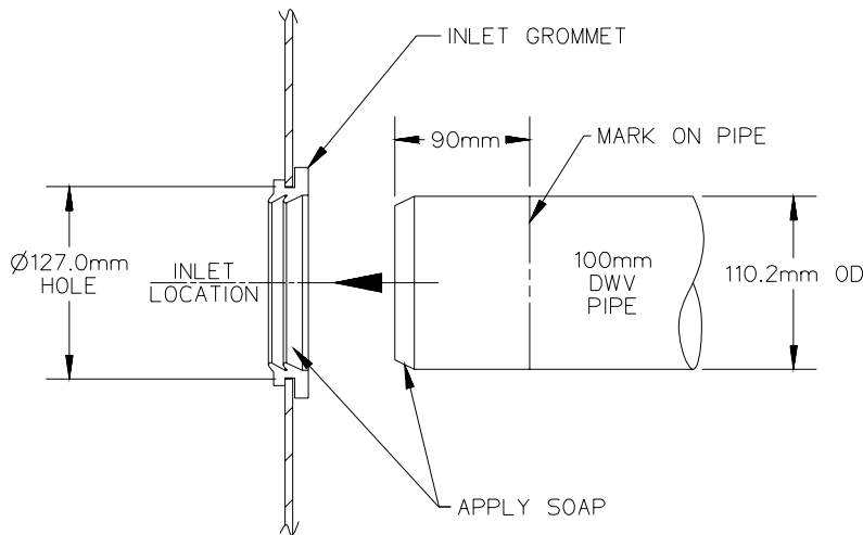
Fig. 5 - Inlet Installation
