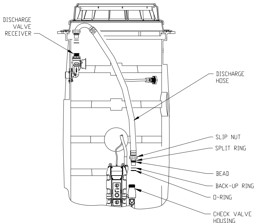
Fig. 9 - Grinder Pump Installation
