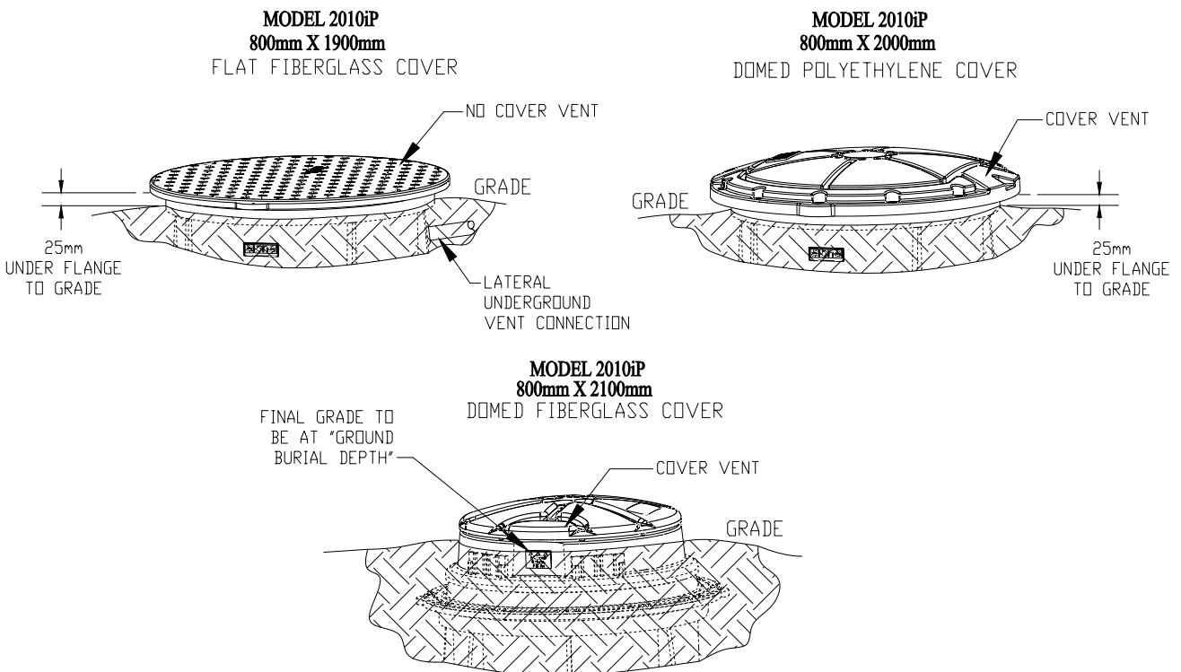
Fig. 4 - Tank Installation
